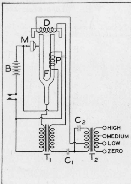
FIGURE 1. Circuit Diagram
